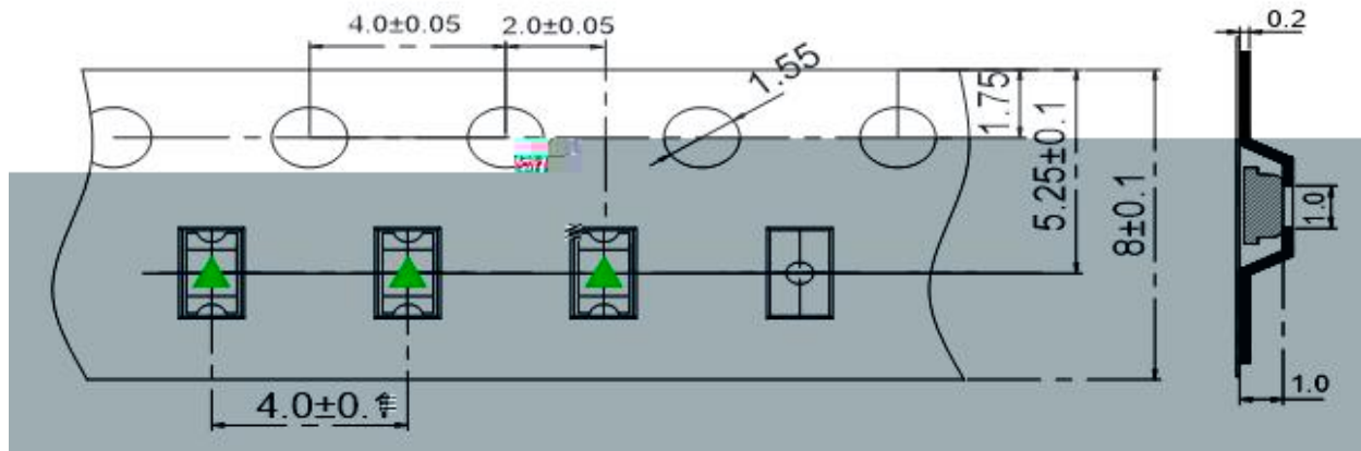
载带与圆盘尺寸 Belt and disk dimensions
