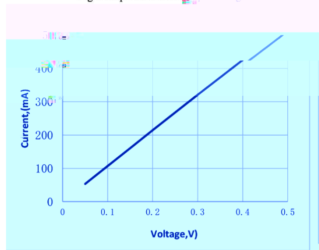
Fig.8 Output current vs. Output voltage
